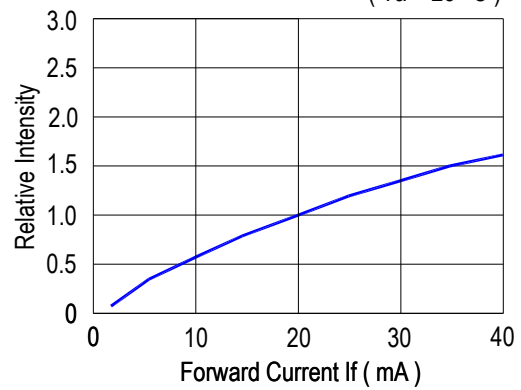
FIG. 2 Relative Intensity vs. Forward Current ( T_a = 25^\circ\text{C} )
