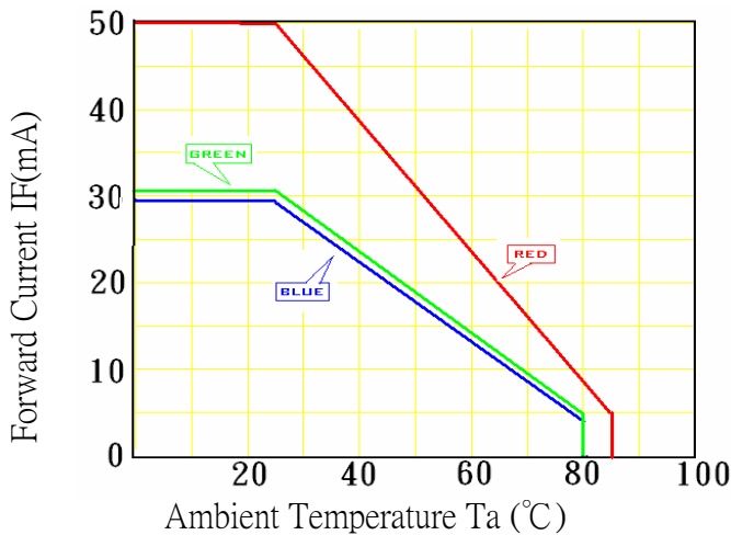
Fig.5 IF-Ta
