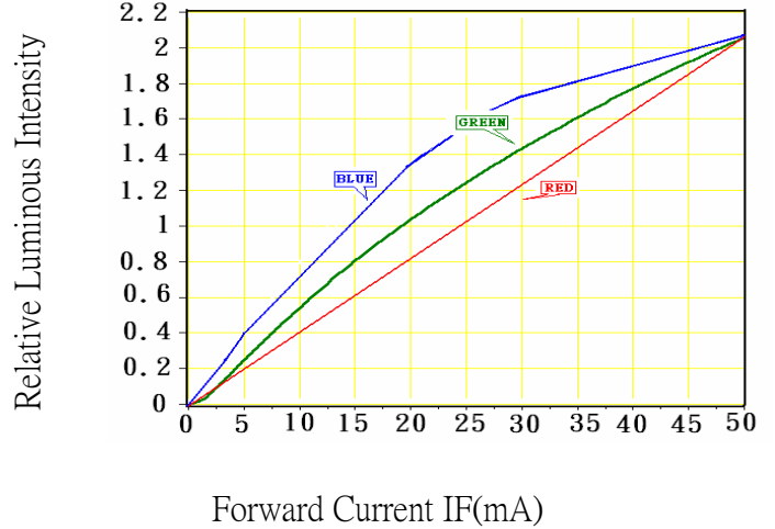
Fig.2 Relative Luminous Intensity-IF (Ta=25°C)
