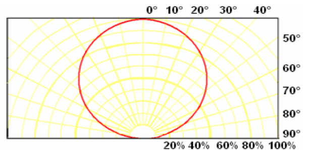
Directive Characteristics (Ta=25°C)
