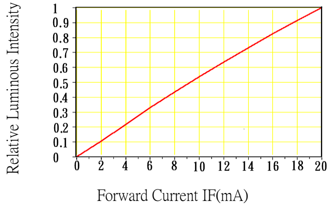
Fig.2 Relative Luminous Intensity-IF (Ta=25°C)
