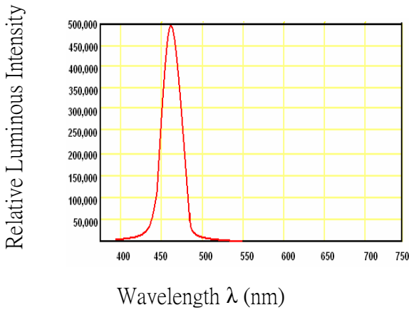
Fig.3 Wavelength Characteristics (Ta=25°C)
