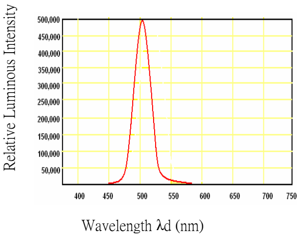
Fig.3 Wavelength Characteristics (Ta=25°C)
