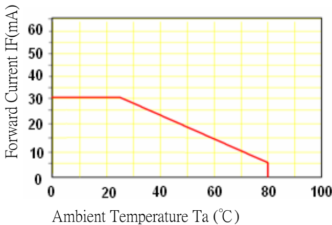
Fig.5 IF-Ta
