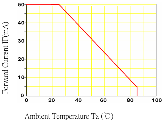
Fig.5 IF-Ta
